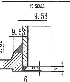
NOZZLE c1 TO FLANGE WELDING DETAIL 接管 c1 与法兰的焊接详图
