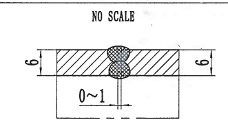
SHELL TO SHELL AND HEAD WELDING DETAIL 筒体与筒体和封头的焊接详图
