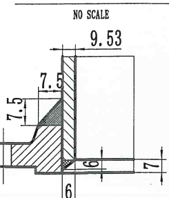
NOZZLE c2 TO FLANGE WELDING DETAIL 接管 c2 与法兰的焊接详图
