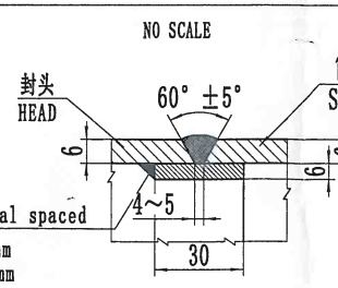
SHELL TO SHELL AND HEAD WELDING DETAIL 筒体与筒体和封头的焊接详图
