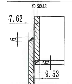
NOZZLE c2 TO NOZZLE WELDING DETAIL 接管 c2 与接管的焊接详图
