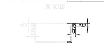
NAMR PLATE SUPPORT TO SHELL WELDING DETAIL 铭牌座与筒体的焊接详图
