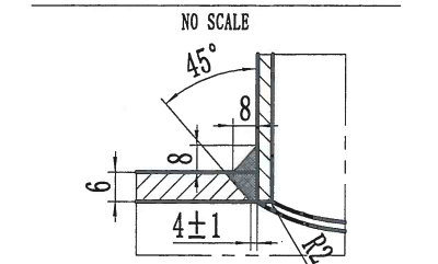
NOZZLE a, b, d TO SHELL AND HEAD WELDING DETAIL 接管 a, b, d 与壳体和封头的焊接详图
